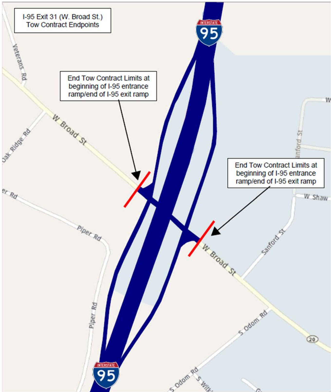
Figure 4: I-95 Exit 31 (W. Broad St.) Interchange
