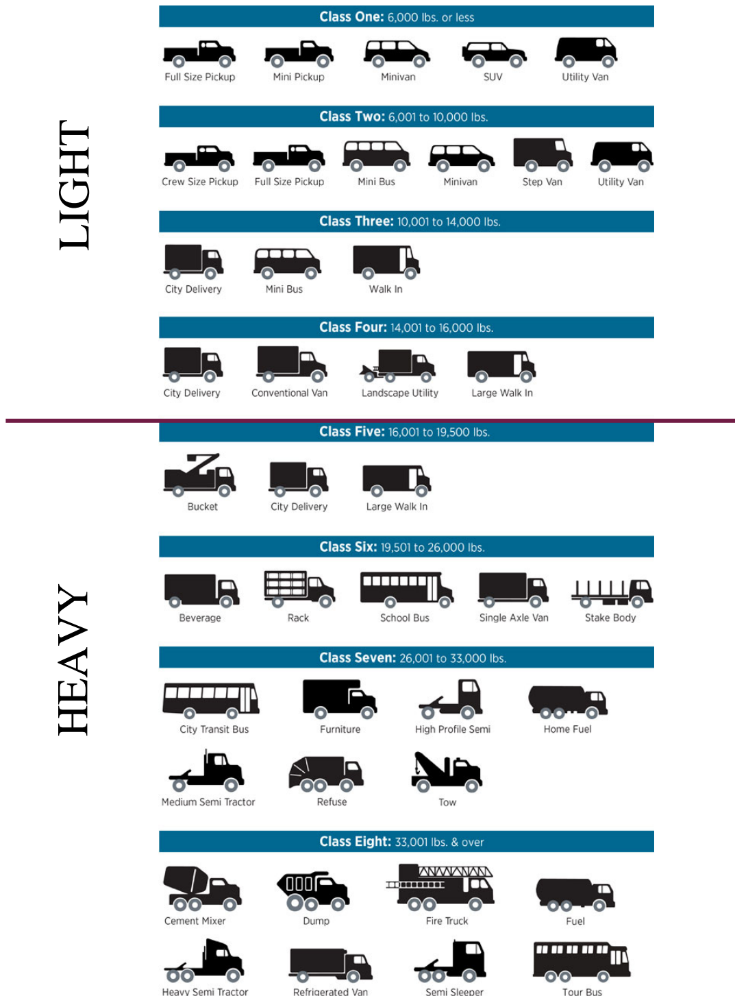
Figure 7: Light and Heavy-Duty Vehicle Classifications
